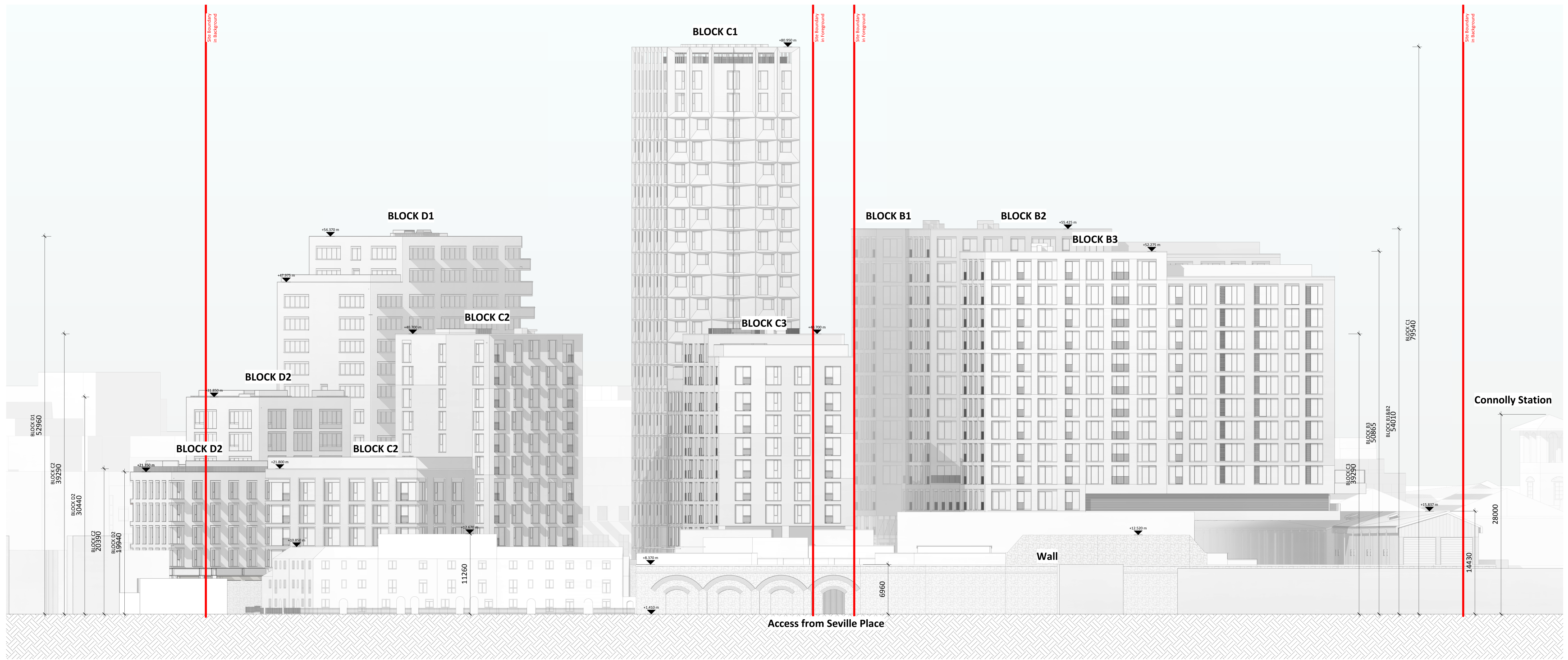
1 Seville Place Elevation - Proposed 1 : 200
